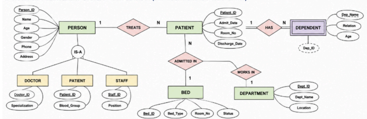
4. HOSPITAL MANAGEMENT SYSTEM – EER DIAGRAM (WITH INHERITANCE AND WEAK ENTITY)
